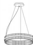
1230S-B Φ780×body H:110 (Max H2000)
