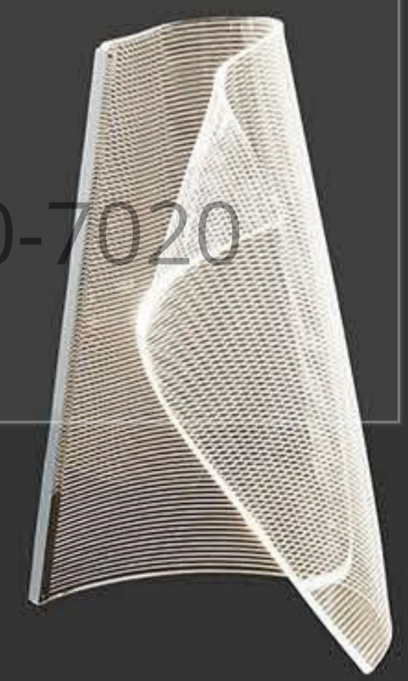
MA05444T-001-06 power : LED 12W 3000K size : W310 H445mm colour : Chrome material : aluminum+Acrylic
