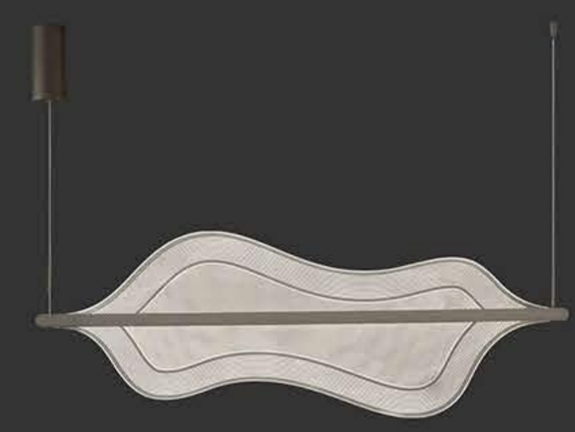
MA05636PA-001 power : LED 42W 3000K size : L1250 W20 H1500mm colour : coffee material : aluminum+iron+Acrylic
