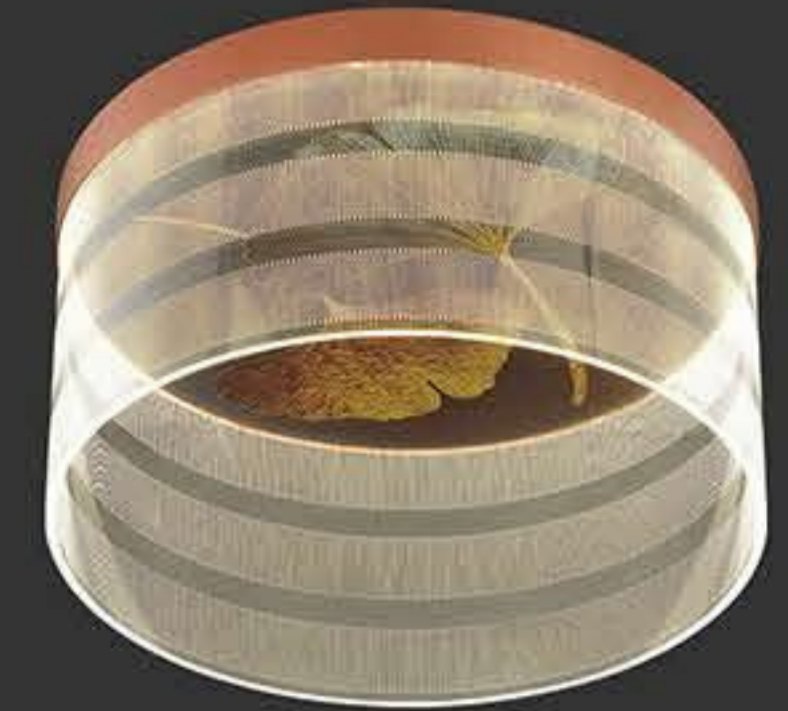
MA05564CA-001 power : LED 25W 3000K size : Φ400 H222mm colour : Goden Red material : iron+Acrylic
