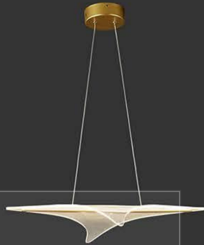
MA05529C-001 power : LED 19W 3000K size : L580 W290 H1500mm colour : gold material : iron+aluminum+Acrylic
