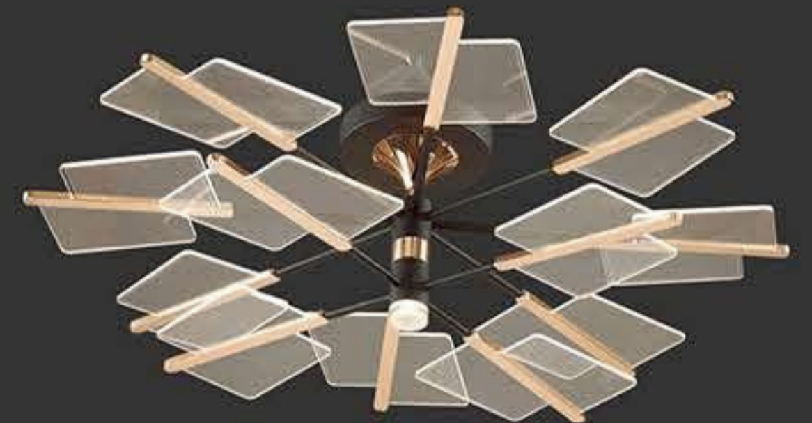
MA05567C-024+2 power : LED 77W 3000K size : \Phi 997 H287mm colour : Goden Red+black material : iron+aluminum+Acrylic
