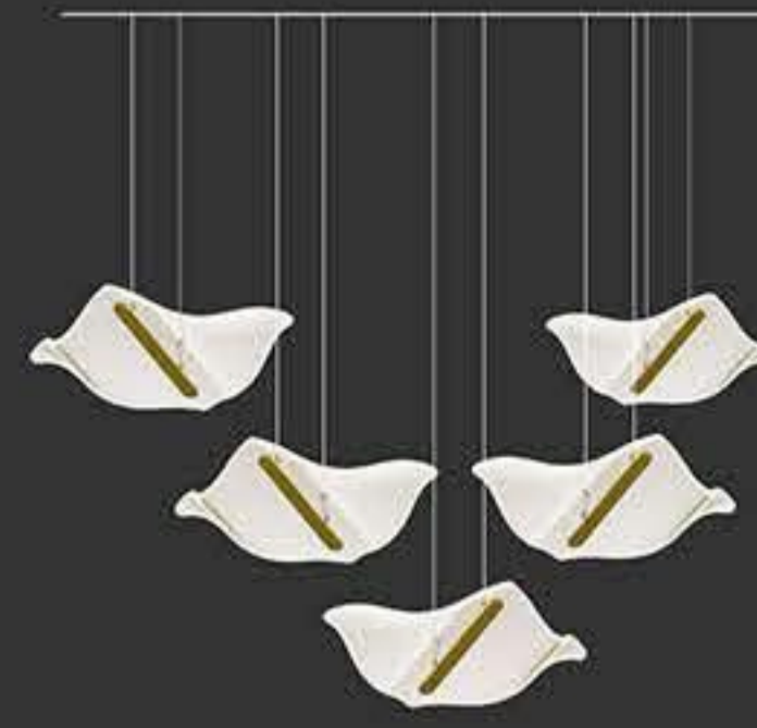
MA05523CC-005 power : LED 40W 3000K size : L1260 W295 H1500mm colour : gold material : istainless steel+aluminum+Acrylic
