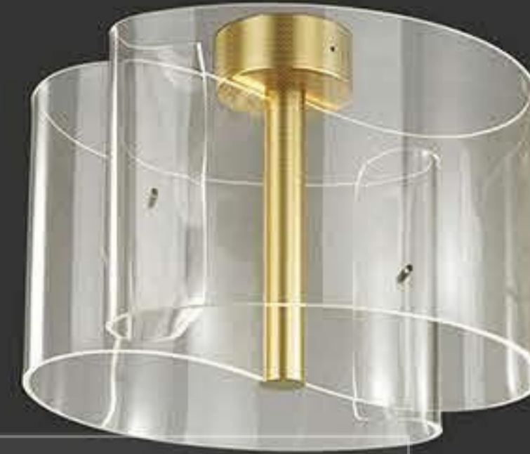
MA0555CA-001 power : LED 16.5W 3000K size : \Phi 460 H305mm colour : gold material : iron+aluminum+Acrylic
