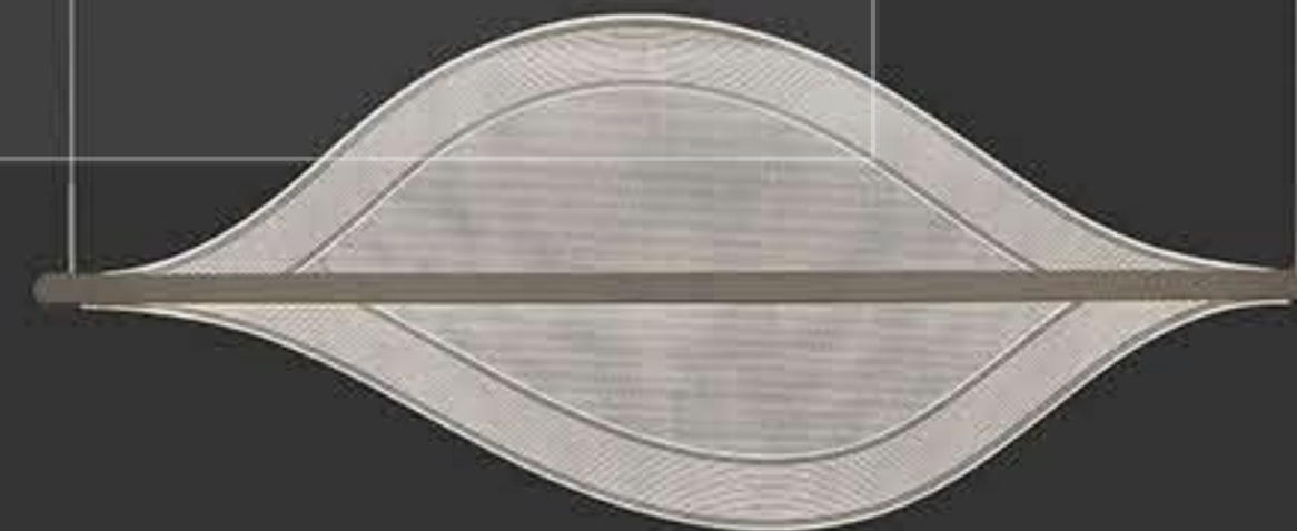
MA05637PB-001 power : LED 56W 3000K size : L1650 W20 H1500mm colour : coffee material : aluminum+iron+Acrylic
